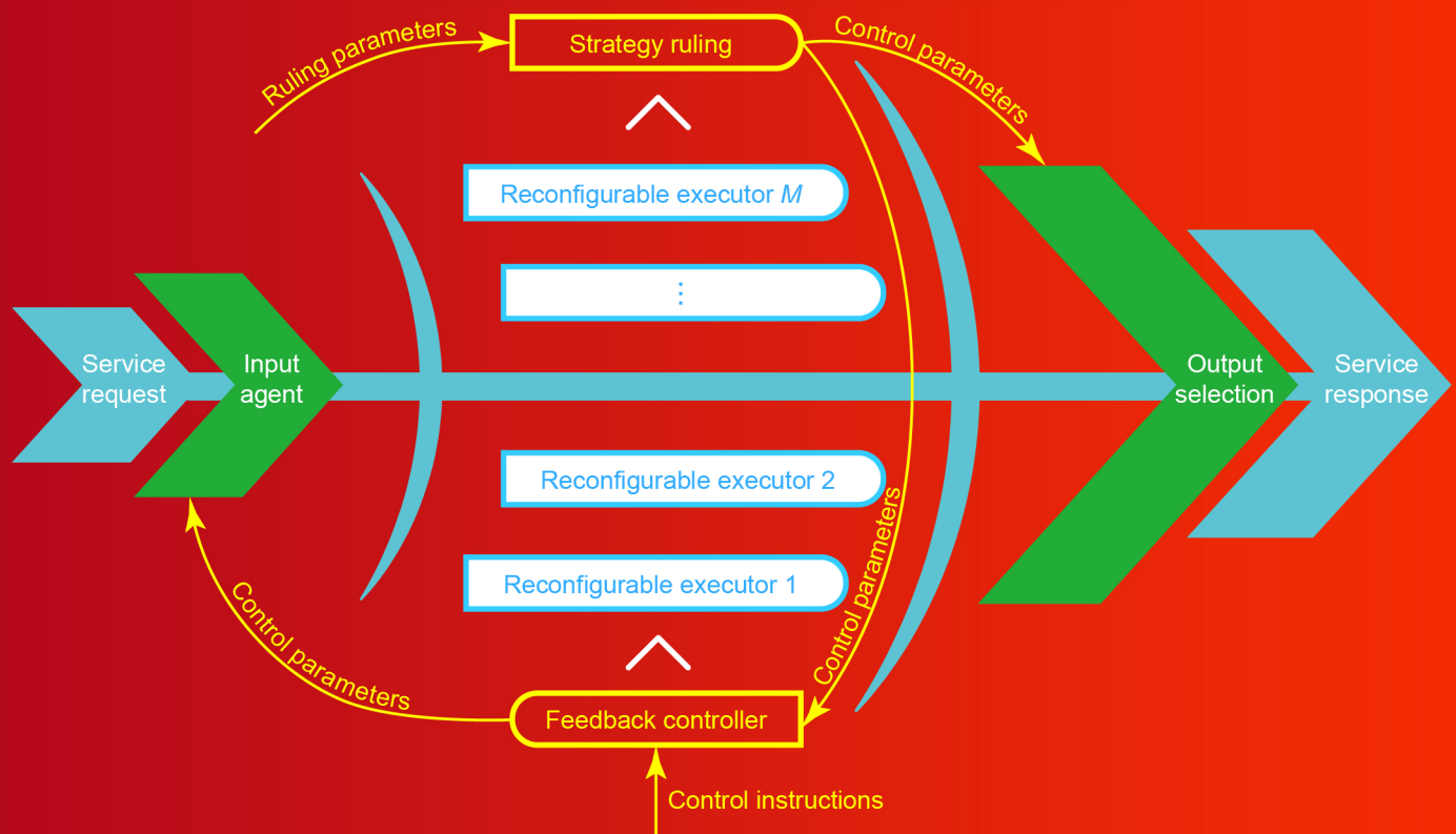
Dynamic heterogeneous redundancy (DHR) structure
