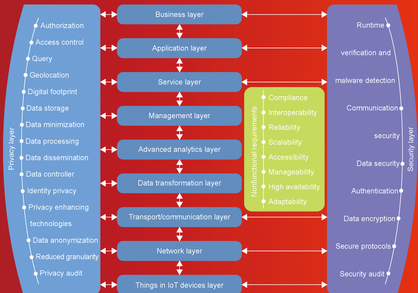
Privacy and security federated reference architecture for Internet of Things Musab KAMAL, Imran RASHID, Waseem IQBAL, et al. https://doi.org/10.1631/FITEE.2200368
