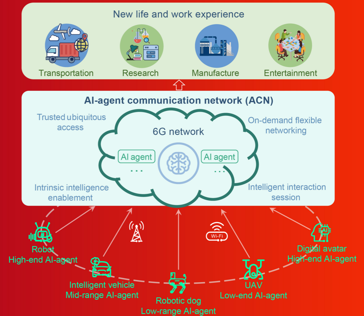
AI-agent communication network for 6G: vision, architecture, and key technologies Xiaodong DUAN, Zhenglei HUANG, Shiyu LIANG, et al. https://doi.org/10.1631/FITEE.2500582
