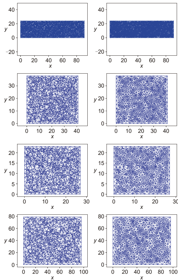
Fig. S1 Examples of meshes in the dataset. For GMSNet, the left column displays meshes used for unsupervised training; whereas for NN-Smoothing model, it takes meshes from the left column as input and from the right column as labels for supervised training
