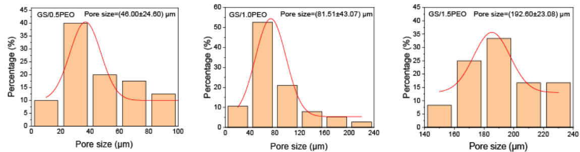
Fig. S1 Quantitative analysis of surface pore size of GS/PEO hydrogel.
