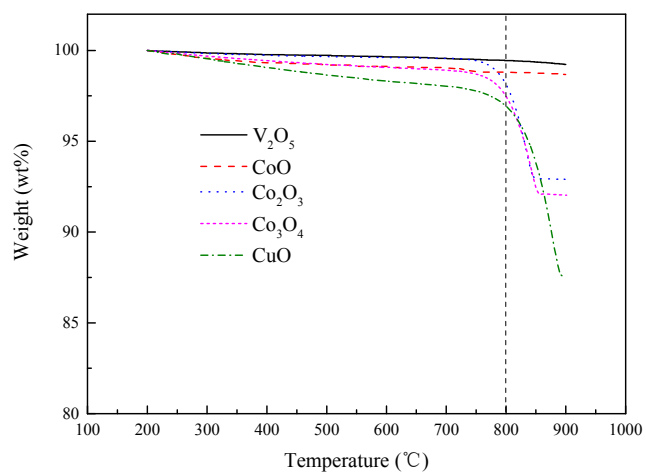
Fig. S1 Thermogravimetric curves of catalysts
