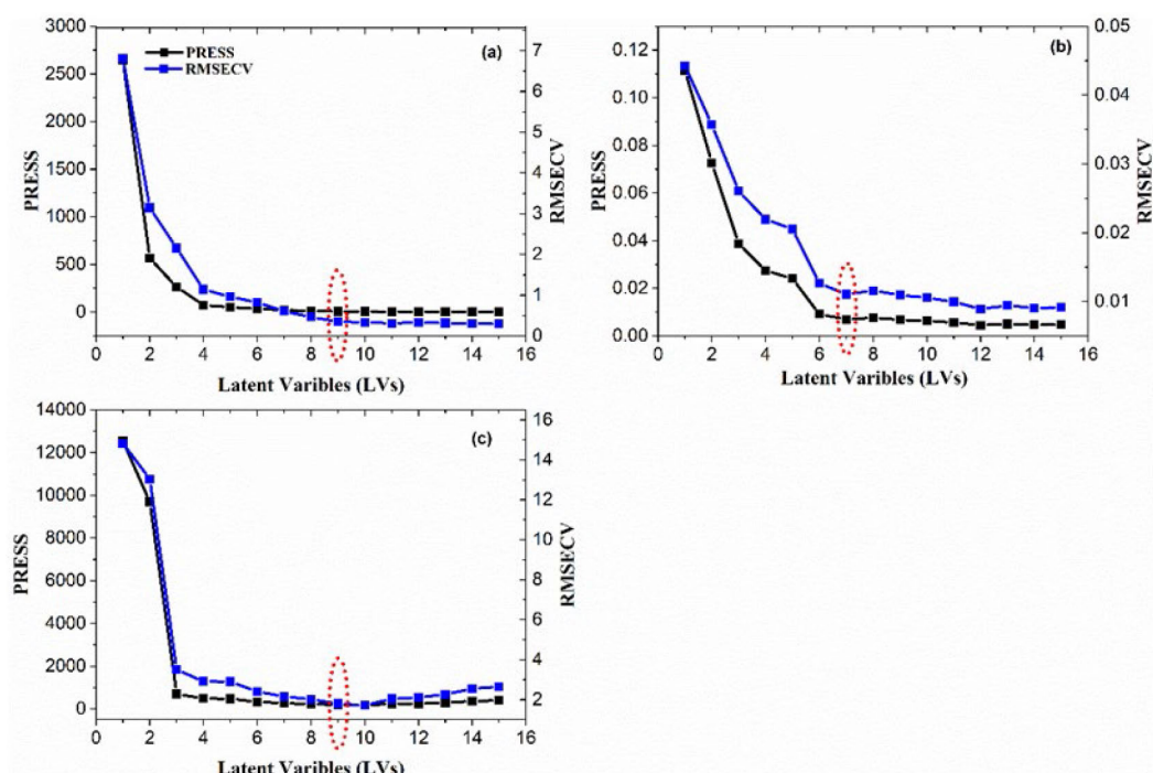
Fig. S1 Scree plot: results of different latent variables for regression models
