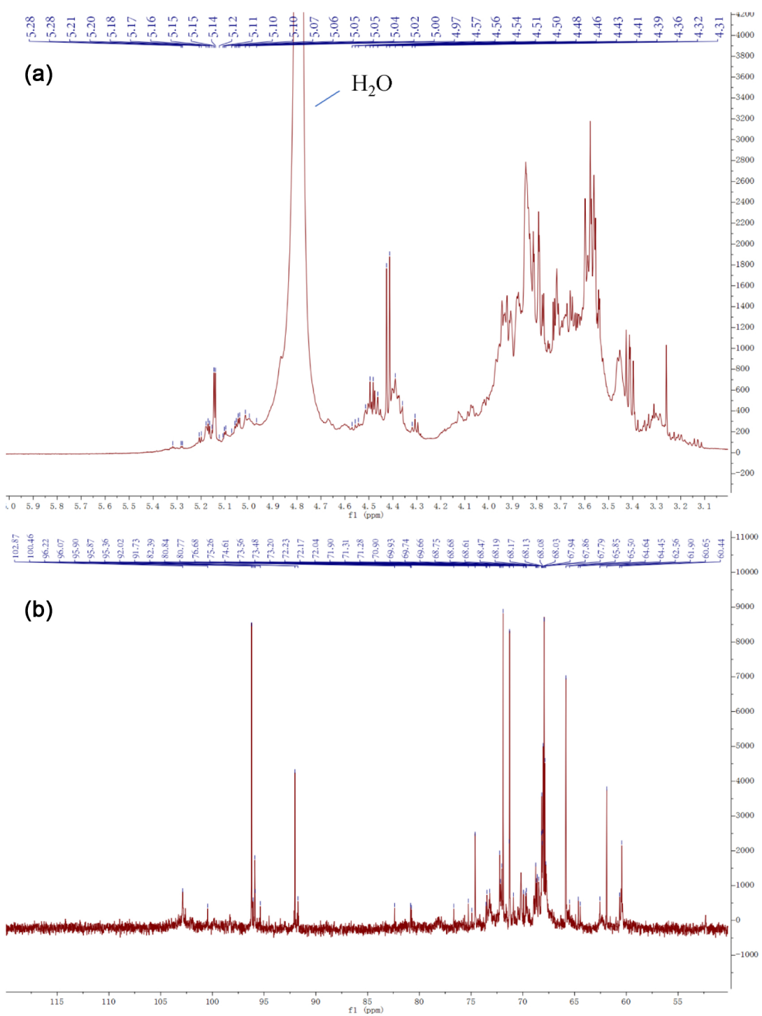
Fig. S1 ^1\text{H} (a) and ^{13}\text{C} (b) nuclear magnetic resonance (NMR) spectra of wax apple polysaccharide (WAP)
