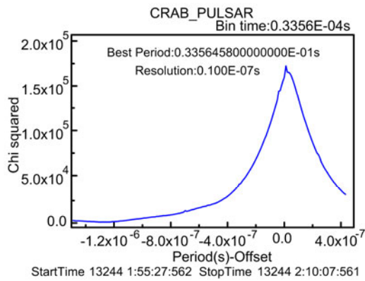
Fig. 1 Period estimation using efssearch in HEASoft
