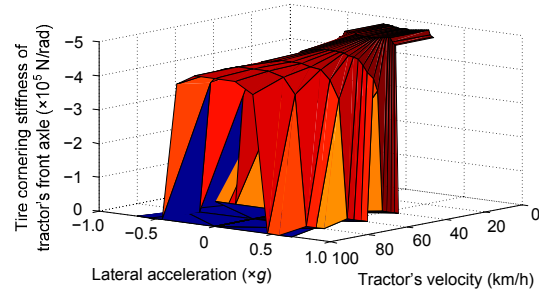
Fig. 2 Tire cornering stiffness of the tractor's front axle
