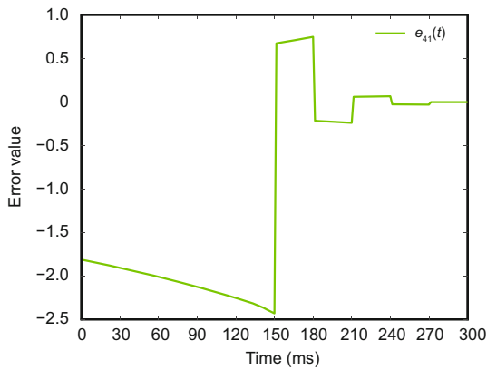
Fig. 11 State error between the fourth agent group and the leader agent
