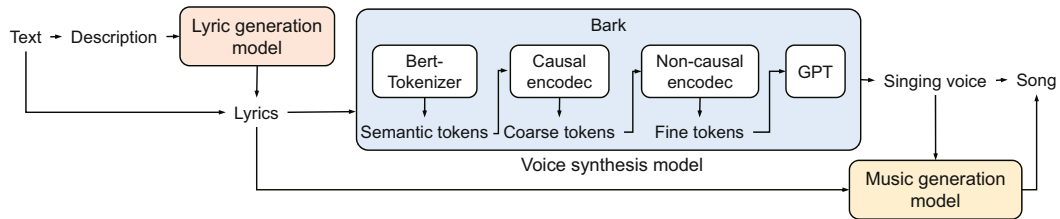
Fig. 2 General framework of AI music generation, including the lyric generation model, the voice synthesis model, and the music generation model
