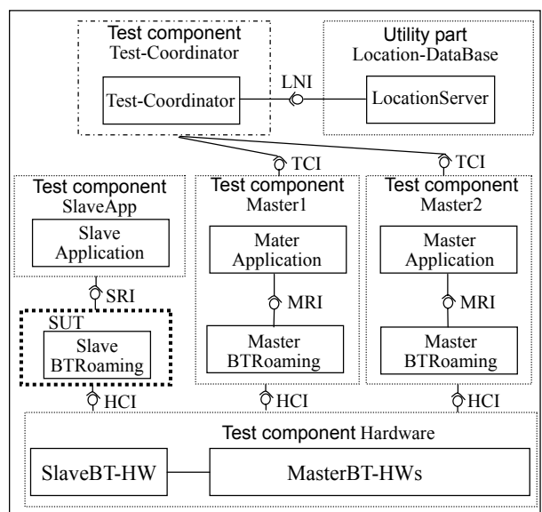
Fig.1 Role Assignment for System Components
