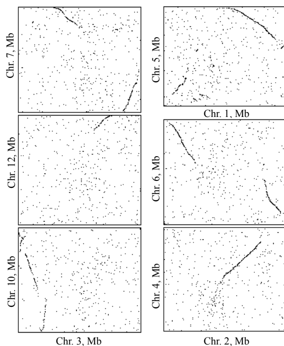
Fig.1 Selected dot-plots of pairs of duplicate genes in the rice genome. Syntenic lines of duplicate blocks corresponding to the latest ancient large-scale duplication (PPP1) are discernible. Pairs of duplicate genes identified as one-to-one paralogs are presented as single dots. The annotation of the TIGR rice assembly ( osa1 , version 2.0) was used
