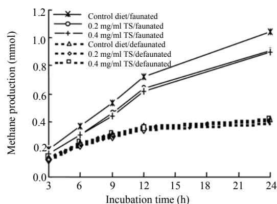
Fig.2 Effect of tea saponin (TS) additon and protozoa status on methane production
