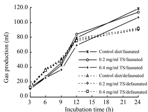
Fig.1 Effect of tea saponin (TS) additon and protozoa status on gas production
