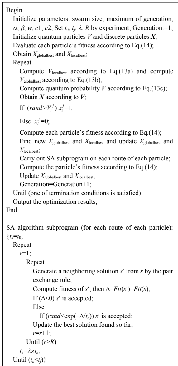
Fig.3 DPSO-SA hybrid optimization algorithm
