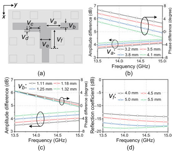
Fig. 6 Geometry and simulation results of the unequal T-junction power divider: (a) geometry; (b) amplitude and phase difference under four different v_a 's; (c) amplitude and phase difference under four different v_b 's; (d) reflection coefficient under four different v_f 's
