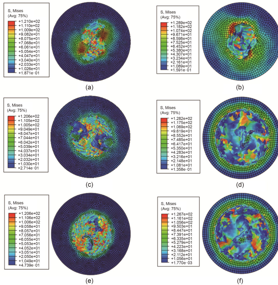
Fig. 7 Equivalent stress diagram of bone tissue. (a, b) 0.25 s; (c, d) 2.5 s; (e, f) 5 s. (a, c, e) Medical twist drill; (b, d, f) Drill-milling tool. Avg: average.
