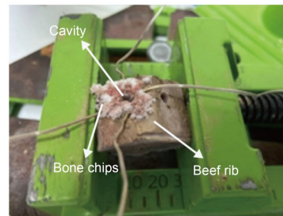
Fig. 10 Bone chips discharged from the cavity.
