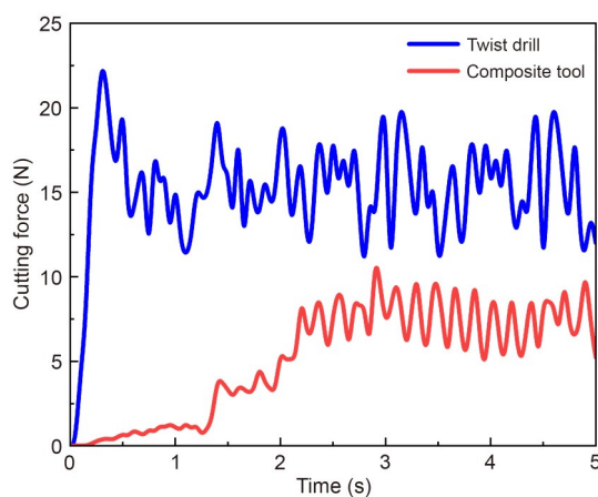
Fig. 8 Axial force variation during the drilling process by twist drill and composite tool.
