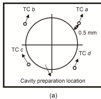
Fig. 6 Thermocouple position. (a) Schematic drawing of thermocouple (TC) distribution (location: TC a–TC d); (b) Bone sample with fixed thermocouple wires.
