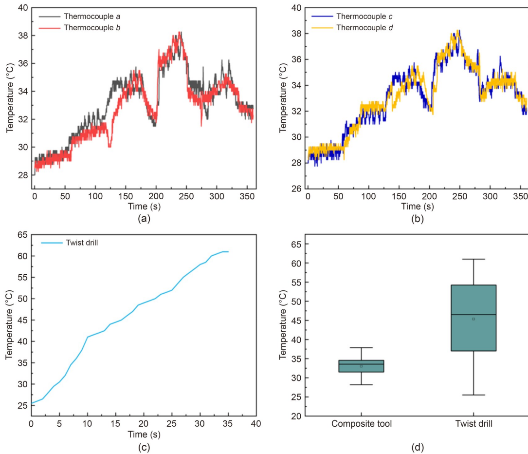
Fig. 9 Temperature change. (a, b) Thermocouple temperature recorded by drill-milling tool; (c) Temperature change recorded by twist drill; (d) Temperature comparison of cavity preparation with different tools.
