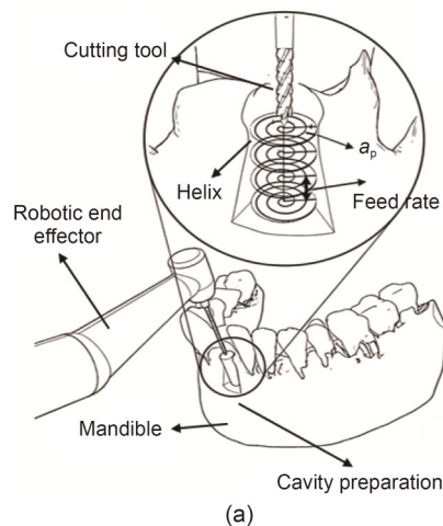
Fig. 4 Schematic diagram of the trajectory planning. (a) Helical milling trajectory; (b) Robotic motion process. a_p : cutting depth.
