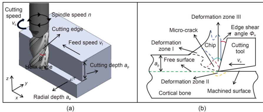
Fig. 1 Milling process. (a) Schematic diagram of the milling operation; (b) Cutting deformation.
