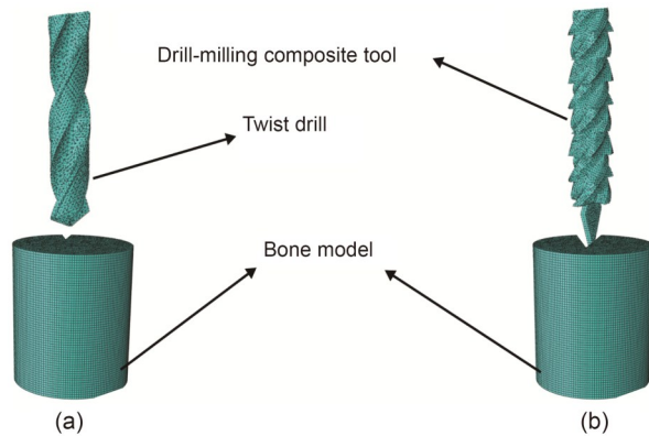
Fig. 3 Tool grid diagram. (a) Twist drill; (b) Drill-milling tool.
