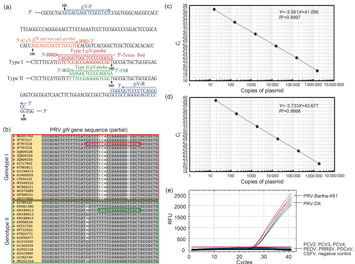
Fig. 1 Diagram of the primers or probes of the gN gene for genotyping of PRV and standard curve or specificity of the TaqMan qPCR assay. (a) Primers and positions of the gN gene for genotyping of PRV. (b) Sequence alignment of gN genes of PRV genotypes I and II. (c, d) Standard curves of the TaqMan qPCR assay of PRV genotypes I (c) and II (d). (e) Specificity of the TaqMan qPCR assay. gN : glycoprotein N; F: forward; R: reverse; Cy5: cyanine 5; BHQ2/3: black hole quencher 2/3; FAM: 6-carboxyfluorescein; MGB: minor groove binder; PRV: pseudorabies virus; C_t : cycle threshold; PCV2/3/4: porcine circovirus type 2/3/4; PEDV: porcine epidemic diarrhea virus; PRRSV: porcine reproductive and respiratory syndrome virus; PDCoV: porcine deltacoronavirus; CSFV: classical swine fever virus; RFU: relative fluorescence unit.
