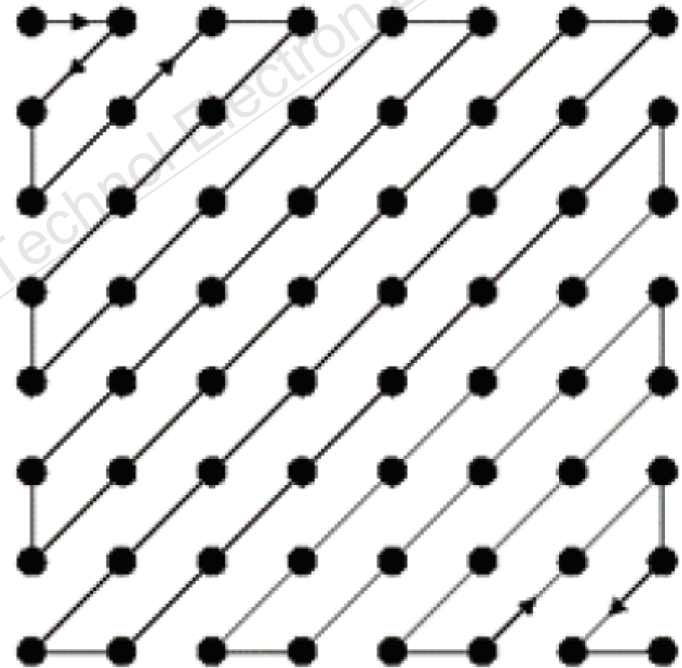
Fig. 2 Zigzag scanning order
