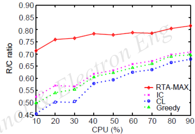
Fig. 8 R/C ratio with increasing CPU
