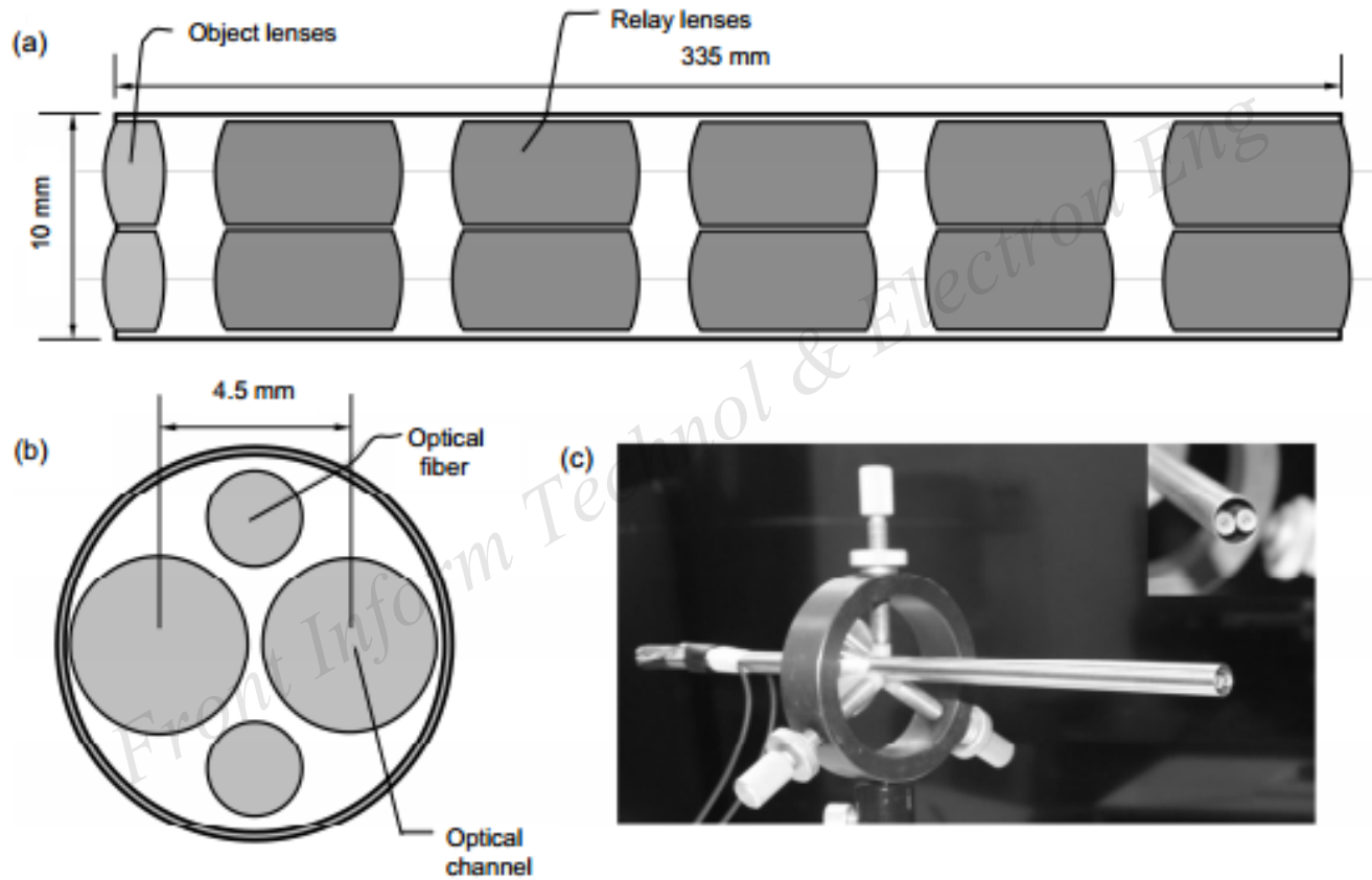
Fig. 1 The optical system of the 3D laparoscope
