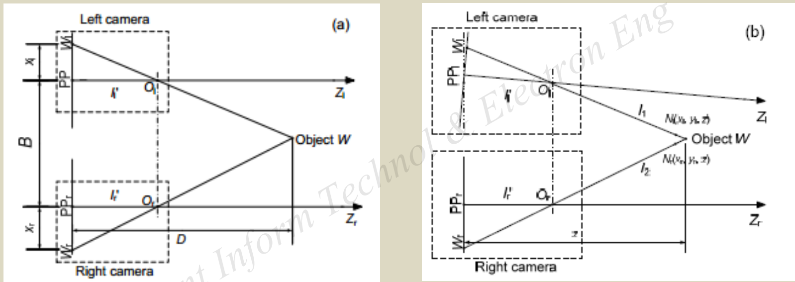
Fig. 2 Ideal (a) and real (b) camera models of laparoscopy O_1 ( O_r ) represents the optical center of the left (right) camera; PP_1 ( PP_r ) represents the principal point of the left (right) camera; W_1 ( W_r ) is the left (right) imaging point of object W
