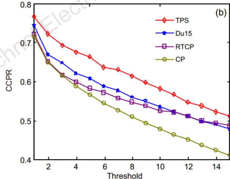
Fig. Comparison of the color contrast preserving ratios (CCPR) obtained by state-of-the-art methods using Cadik's dataset (a) and the CSDD dataset (b).
