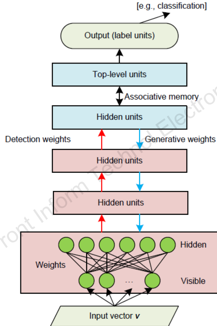
Fig. 5 The framework of deep belief networks
