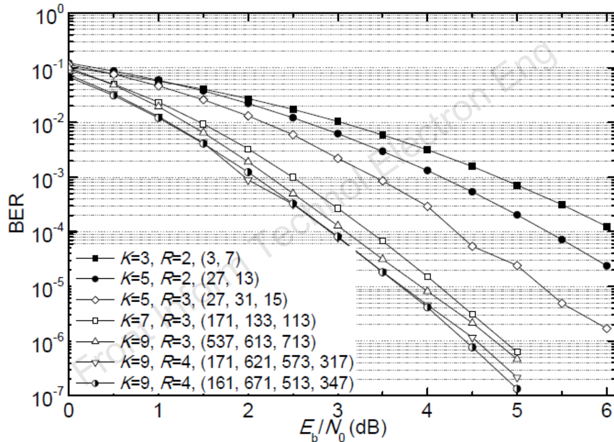
Fig. 5 Bit error rate of the proposed architecture The numbers in parentheses indicate the polynomials in octal format
