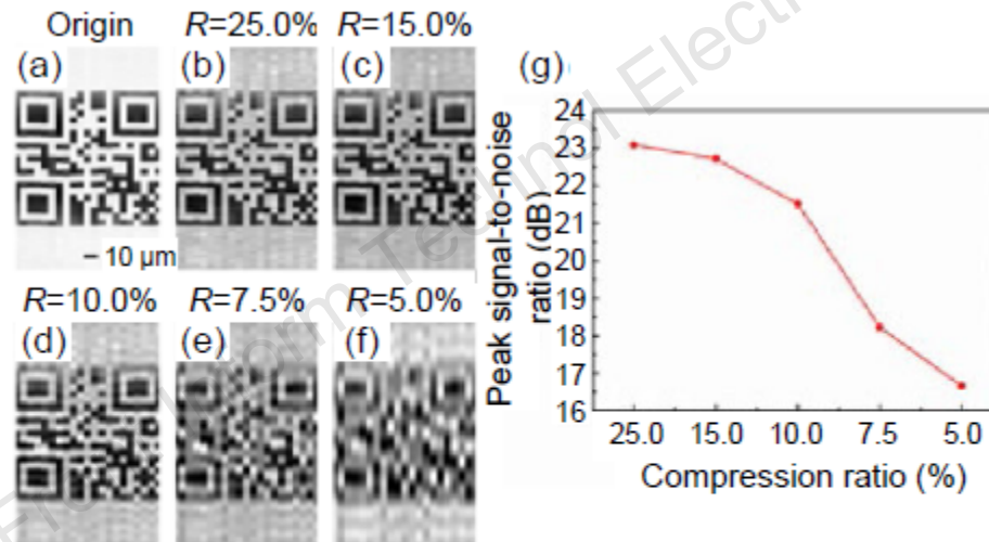
Fig. 3 Surface inspection: (a) original image of a quick response code; (b)–(f) reconstructed images at compression ratios of 25.0%, 15.0%, 10.0%, 7.5%, and 5.0%, respectively; (g) peak signal-to-noise ratio versus compression ratio curve
