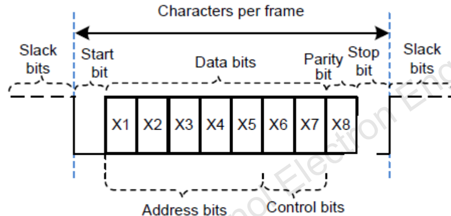
Fig. 5 Definition of the communication protocol
