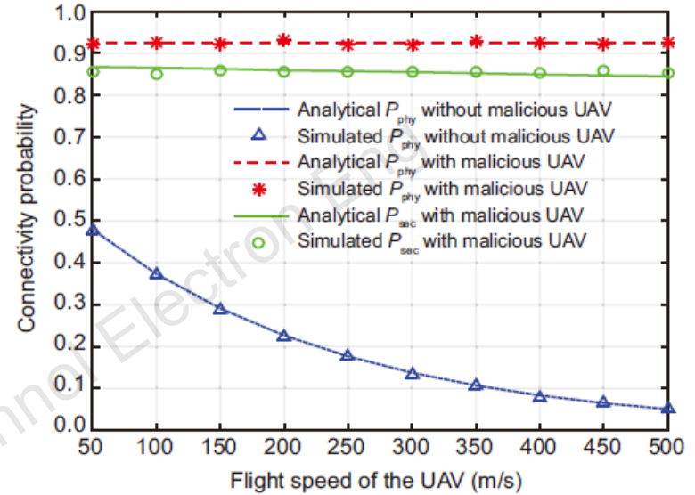
Fig. 12 The relationship between the connectivity probability and flight speed of the UAV V
