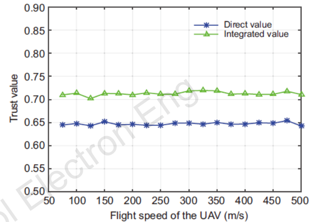
Fig. 8 Robustness of the proposed trust model against mobility
