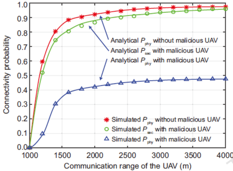
Fig. 11 The relationship between the connectivity probability and communication range r_{th}
