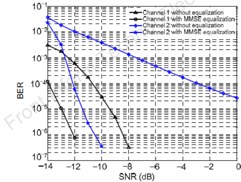
Fig. 8 Simulation results of channel estimation and equalization for different channels
