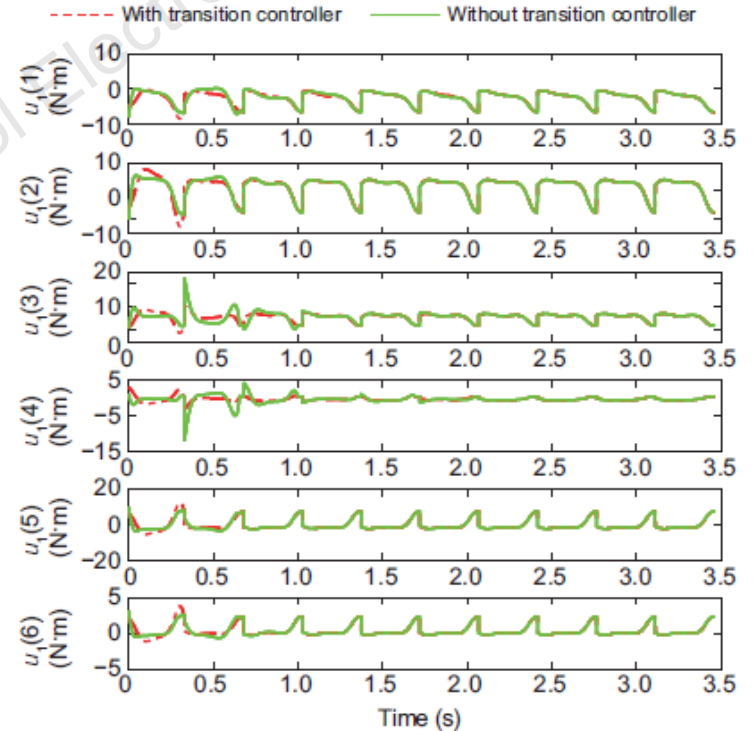
Fig. 6 Torques required for gait transition. The peak values of the torques with and without the transition controller are 12.5 and 22.1 N·m, respectively
