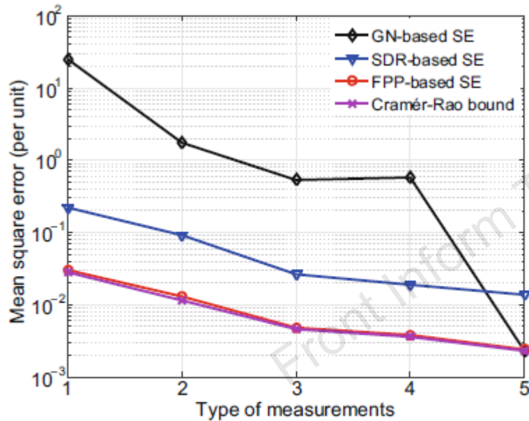
Fig. 1 MSE and Cramér-Rao bound versus the type of measurements used for the IEEE 14-bus system
