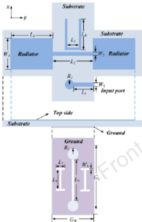
Fig. 6 Configuration of an omni-directional filtering dipole antenna Reprinted from Zhang Y et al. (2018), Copyright 2018, with permission from IEEE
