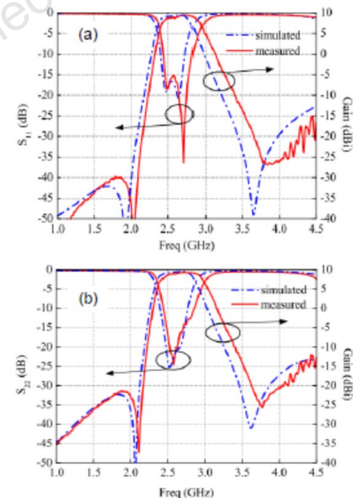
Fig. 4 Reflection coefficients and gain curves: (a) port 1; (b) port 2 Reprinted from Duan et al. (2016), Copyright 2016, with permission from IEEE
