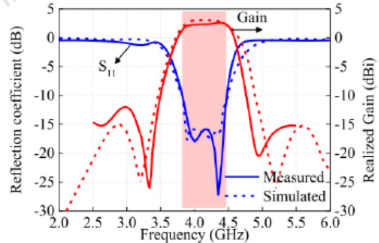
Fig. 7 Measured reflection coefficient and realized gain of the proposed omni-directional filtering dipole antenna Reprinted from Zhang Y et al. (2018), Copyright 2018, with permission from IEEE
