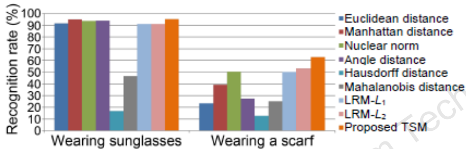
Fig. 15 Average recognition rate on the AR database with real face disguise
