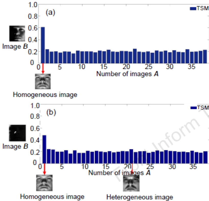
Fig. 4 An intuitive illustration of the insensitivity of TSM to the illumination variation conditions: (a) extreme illumination condition 1; (b) extreme illumination condition 2
