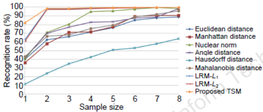
Fig. 12 Average recognition rate on the CMU PIE face database
