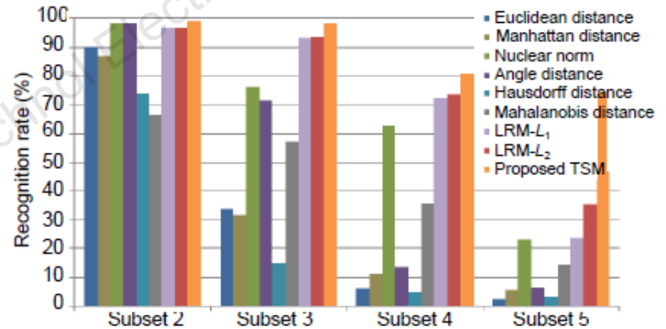
Fig. 11 Recognition rate on the Extended Yale B database under various lighting conditions
