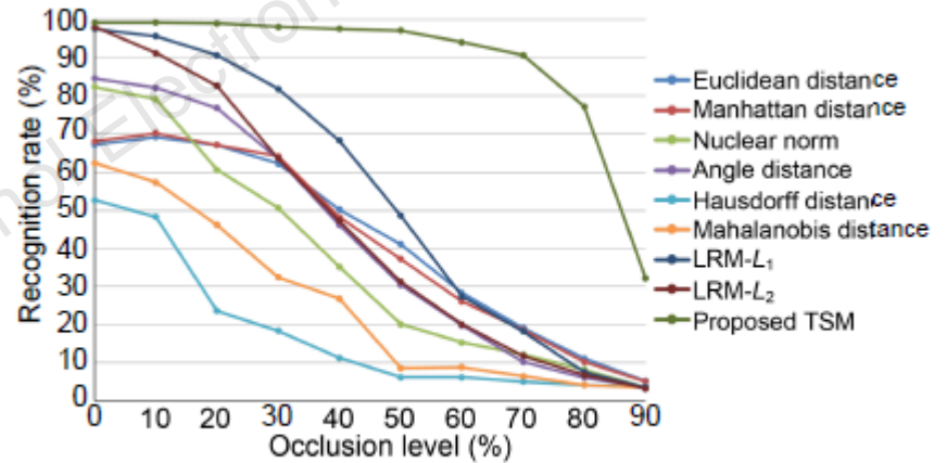
Fig. 14 Recognition rate under different occlusion levels
