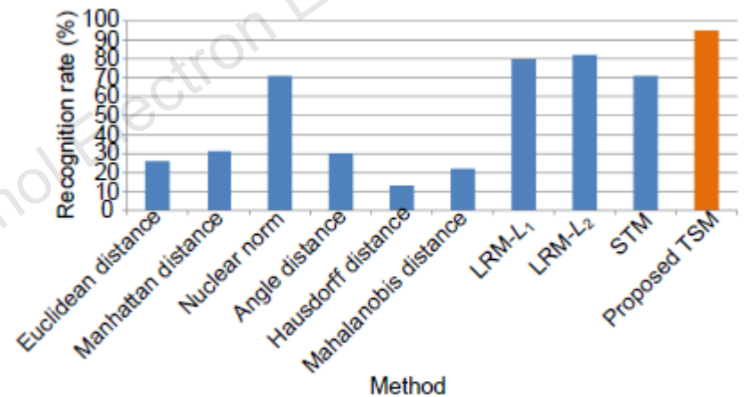
Fig. 16 Recognition rate on the CUHK sketch face database
