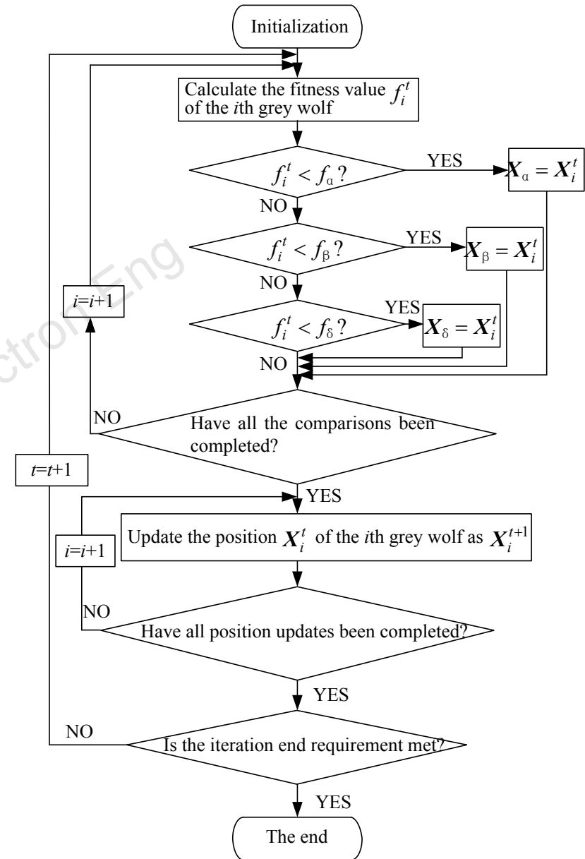
Fig. 5 Flow chart of the static GWO
