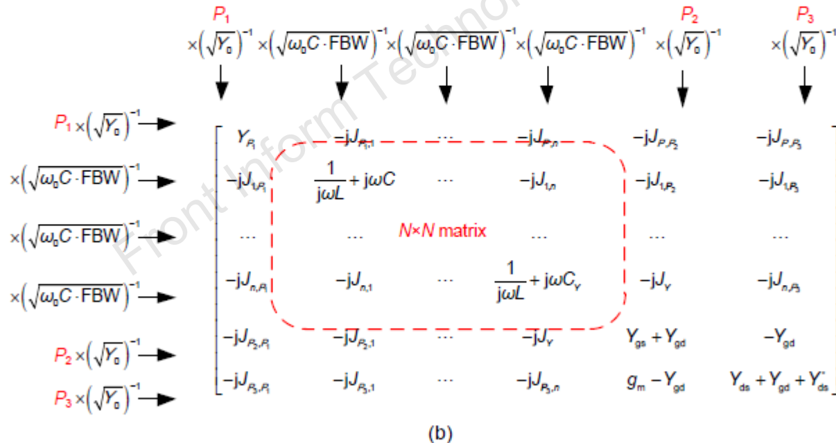
Fig. 2 Simplified lumped circuit of the filter direct-coupled amplifier (a) and matrix [Y] of the lumped circuit and matrix scaling operation from [Y] to [\bar{Y}] (b)
