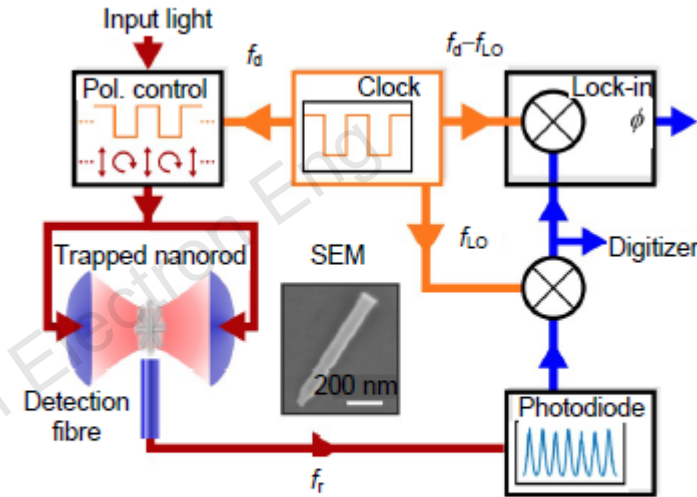
Fig. 8 Scheme of frequency locking experiment
