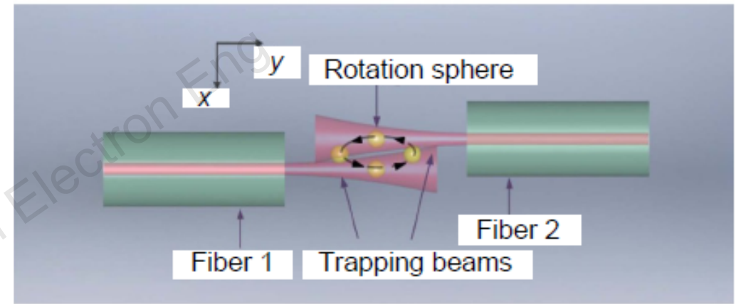
Fig. 1 Rotating particle by misalignment along the radial axis
