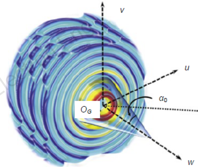
Fig. 5 Wavefront of Bessel beam
