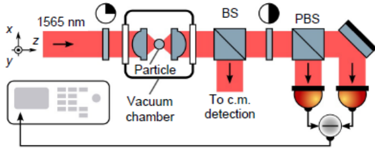
Fig. 6 Experimental setup in Reimann et al. (2018)'s research
