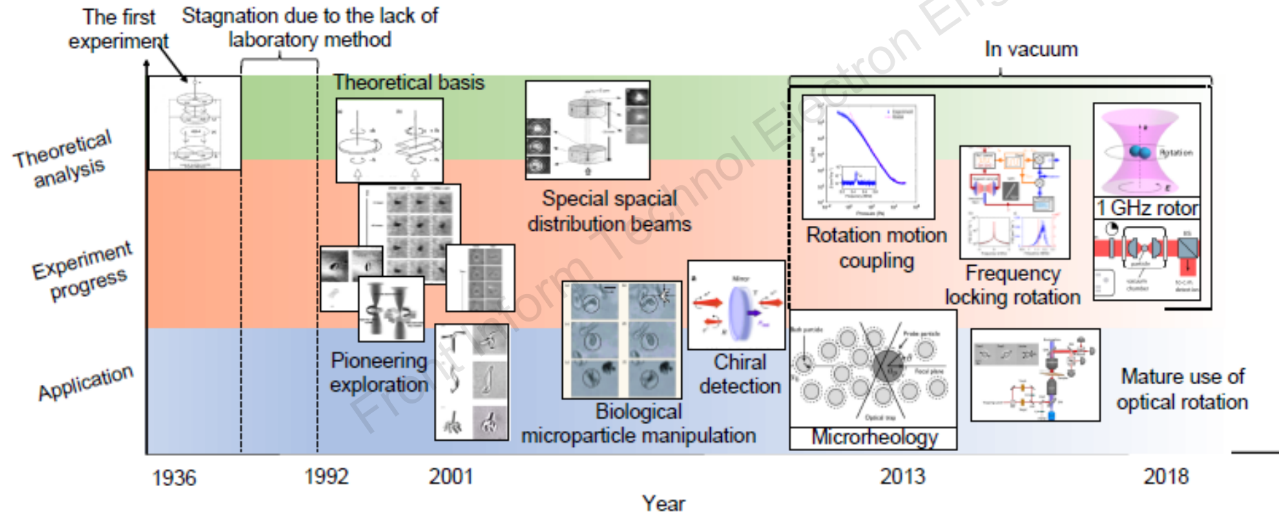
Fig. 9 Development history of optical rotation
