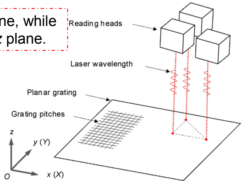
Fig. 4 Benchmarks of a typical six-DOF grating interferometer
