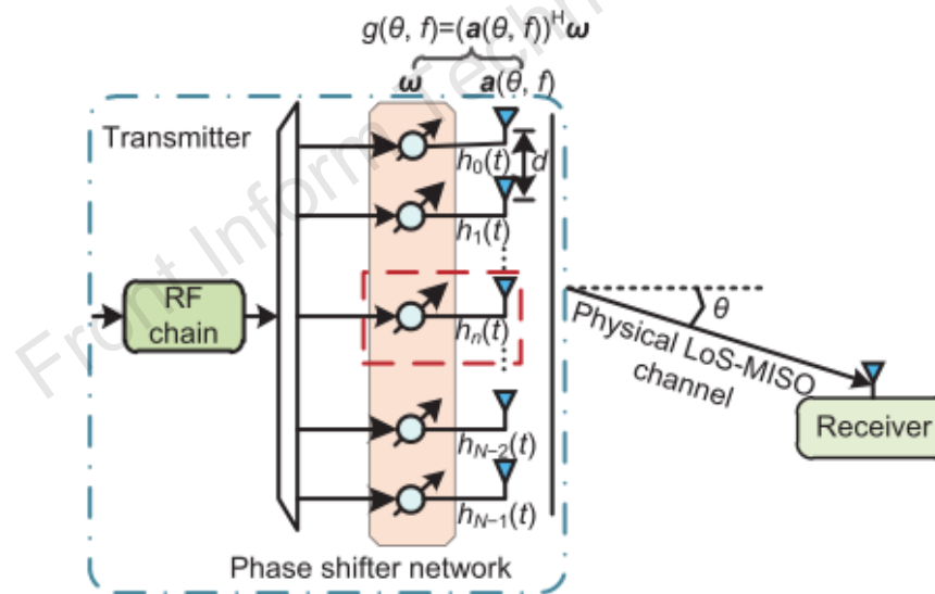
Fig. 1 Model of a line-of-sight multiple-input single-output (LoS-MISO) system where the transmitter deploys an ultra-massive phased array
