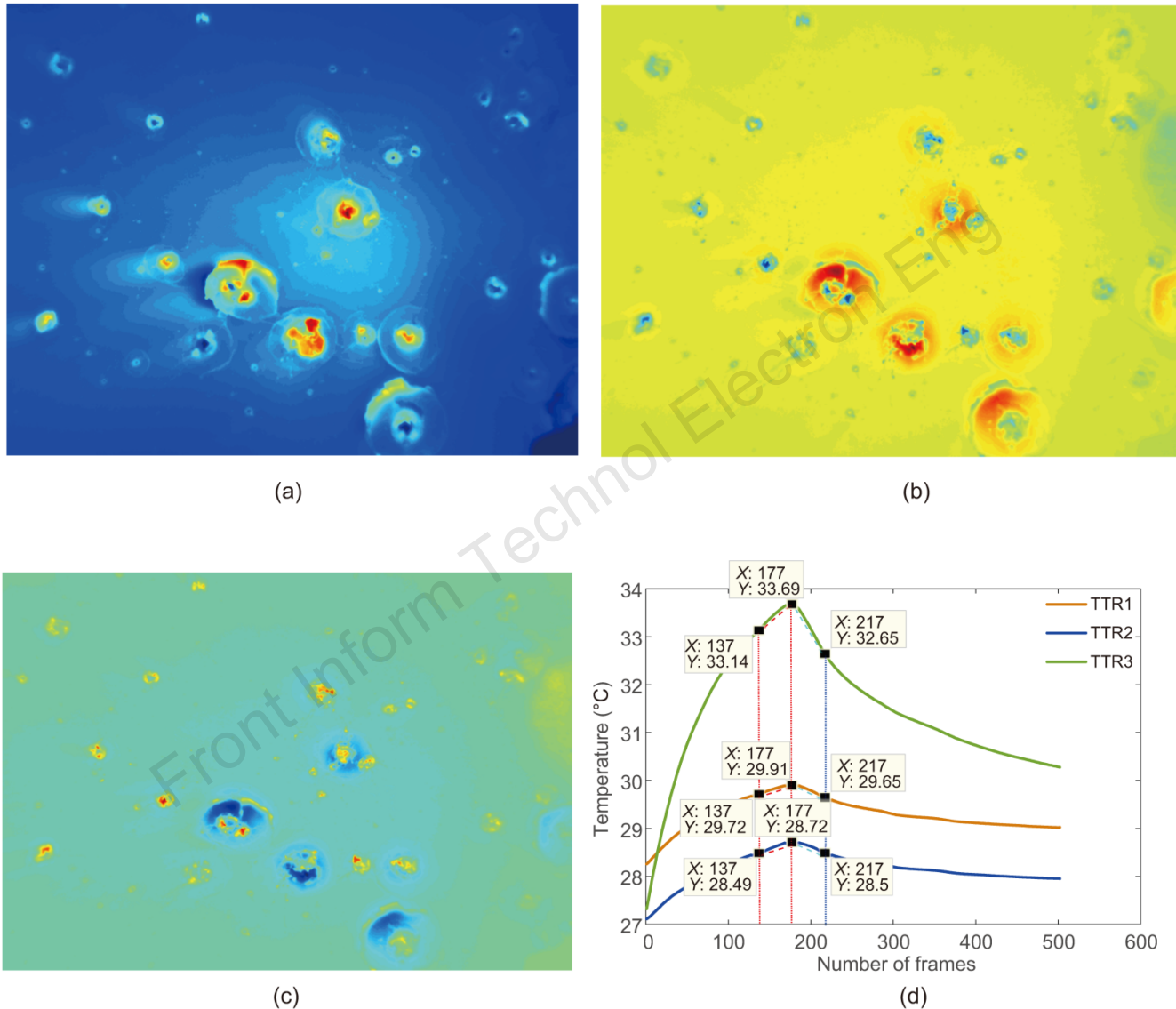
Fig. 9 IRRI acquisition results for the sample: (a) stress damage around the perforation defect; (b) drum kit; (c) perforation damage; (d) TTR for damage
