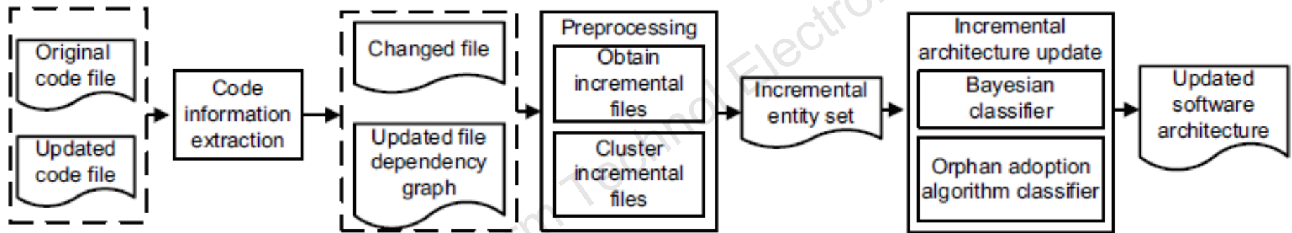
Fig. 1 Incremental software architecture recovery (ISAR) framework
