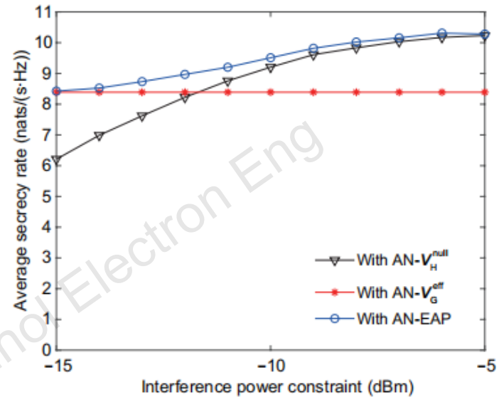
Fig. 10 Average secrecy rate of the large-dimensional C-MIMO system via V_H^{\text{null}} , V_G^{\text{eff}} , and the simplified EAP methods when K=64 , N_B=4 , N_E=2 , N_P=2 , r=3 m, e_0=10 m, and \Gamma_s=13 dBm (C-MIMO: cooperative multi-input multi-output; EAP: eigenspace-adaptive precoding)
