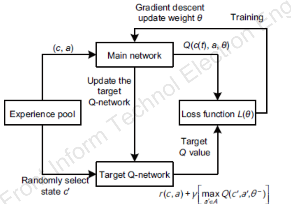
Fig. 3 Deep Q-learning network training model
