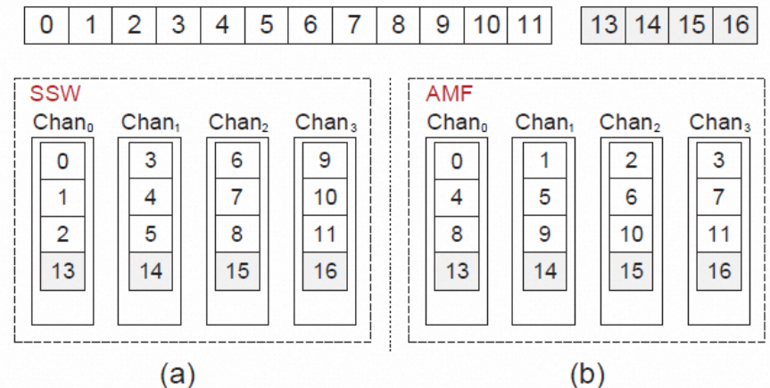
Fig. 9 Data placement strategies in SSW (a) and AMF (b). Chan: channel
