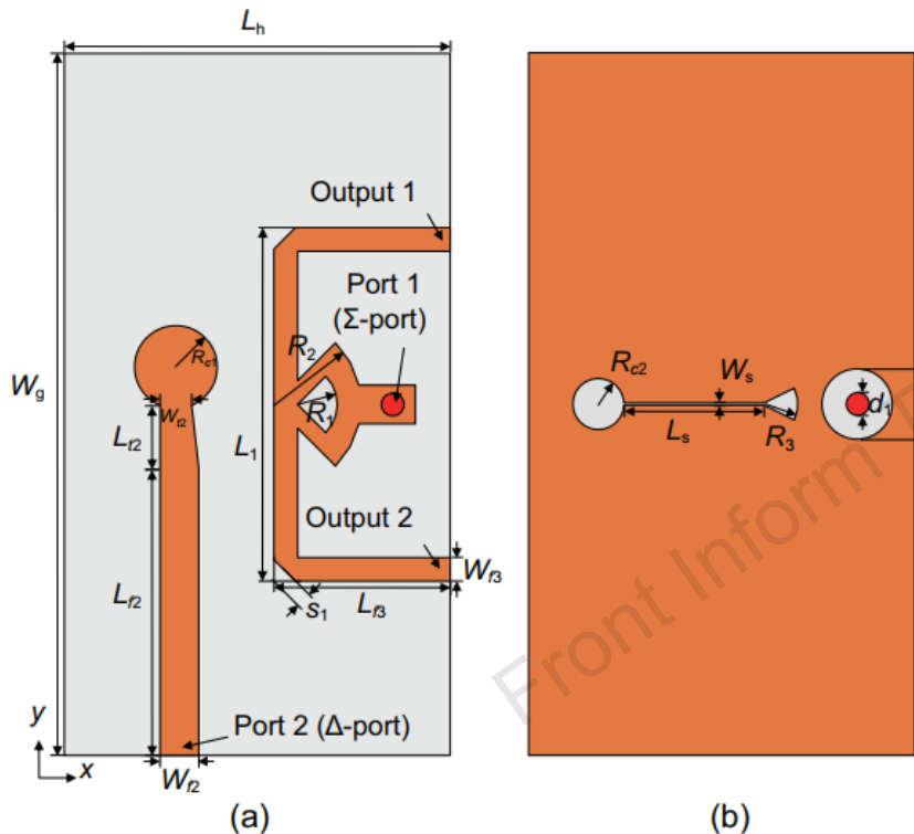
Fig. 2 Geometry of the wideband 180^\circ hybrid: (a) top view; (b) bottom view
