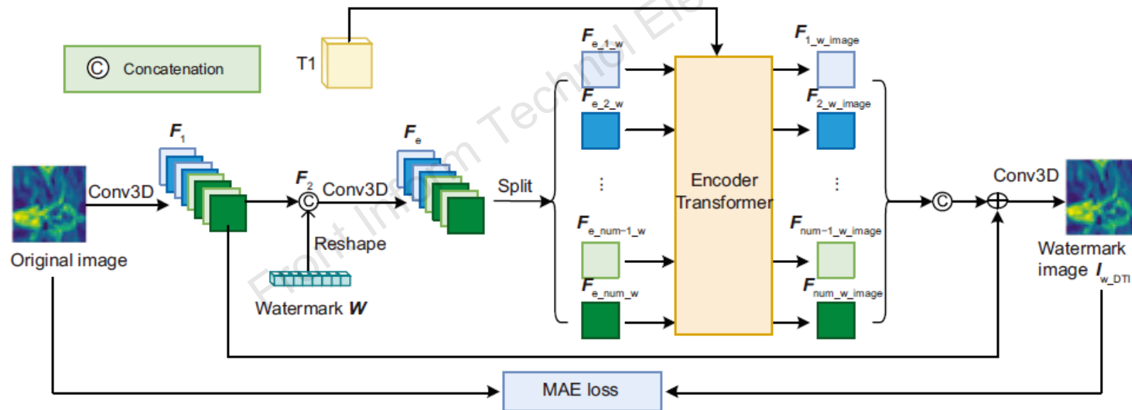
Fig. 2 Watermark-embedding network
