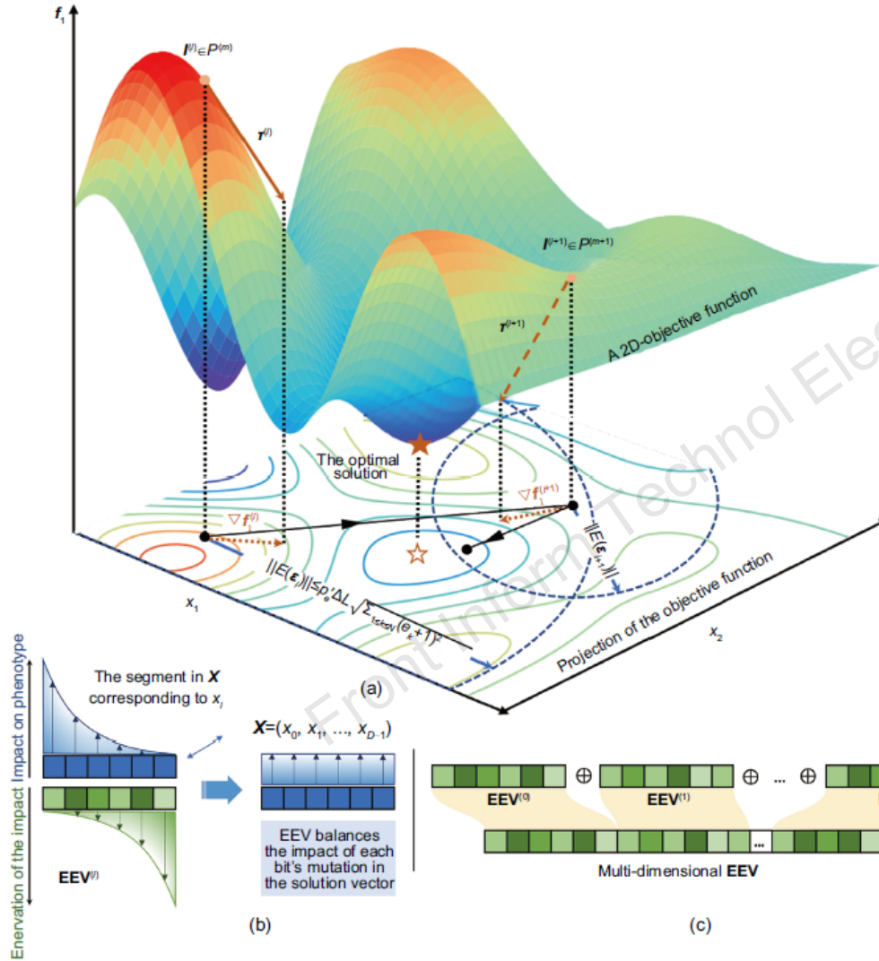
Fig. 3 Three steps for establishing a multi-dimensional environmental vector of probabilistic environmental gradient (PEG) to regulate evolution: (a) computation of gradients for searches based on PEG; (b) establishment of an exponential environmental vector (EEV) with the guidance of PEG; (c) aggregation of the multi-dimensional exponential environmental vector (MEEV) ( P^{(m)} denotes the population at the m^{\text{th}} generation)
