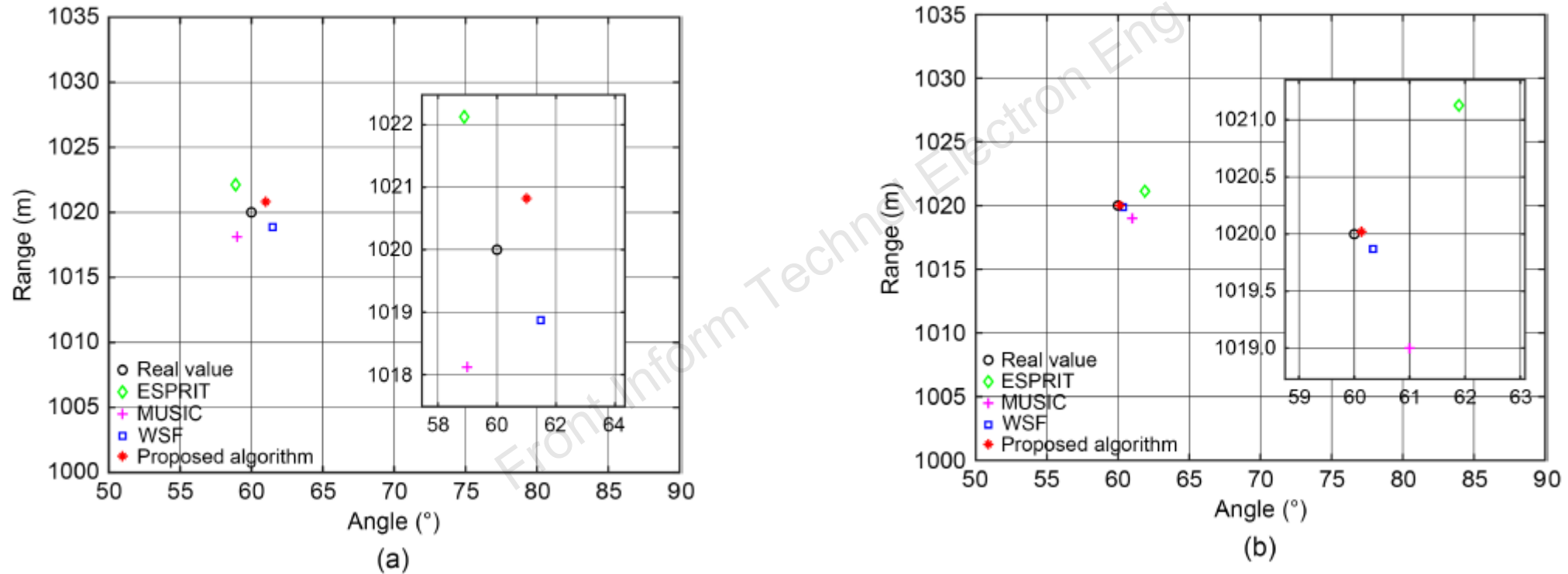
Fig. 1 Comparison of the target parameter estimation results for SNR=-5 dB (a) and SNR=5 dB (b) (SNR: signal-to-noise ratio)
