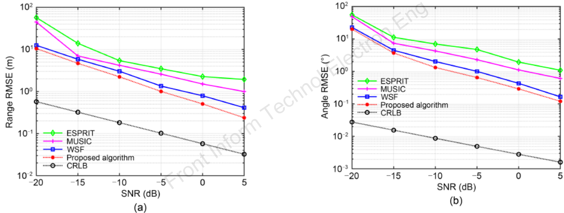
Fig. 2 Multi-target estimation performance versus SNR: (a) range estimation RMSE versus SNR; (b) angle estimation RMSE versus SNR (SNR: signal-to-noise ratio; RMSE: root mean square error)
