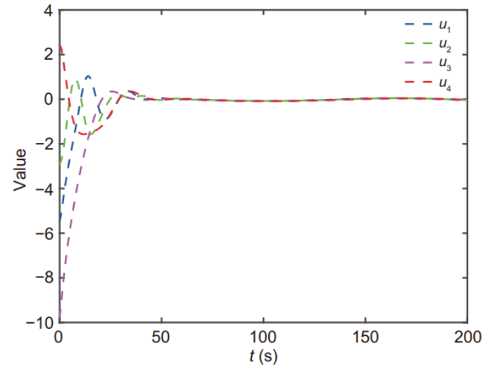
Fig. 8 Control inputs in Example 1
