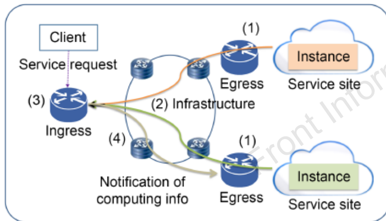
CATS based on distributed control
