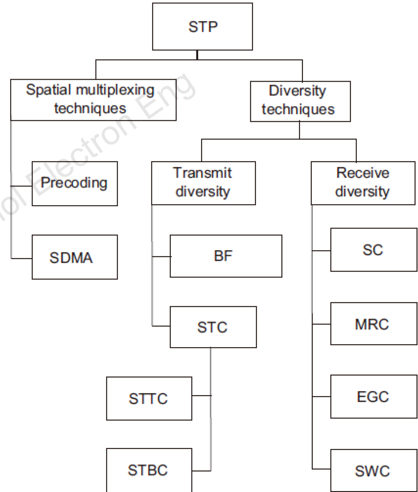
Fig. 4 Categories of STP techniques
