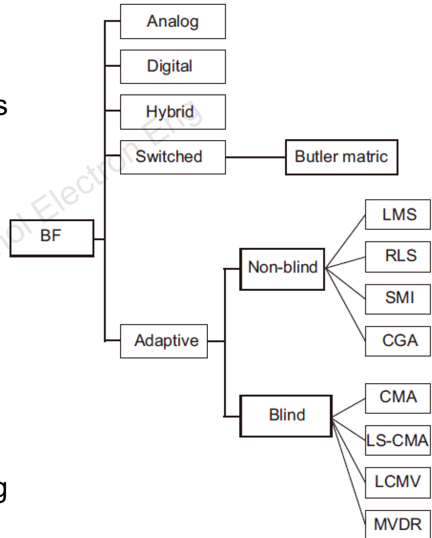
Fig. 12 Classification of BF techniques
