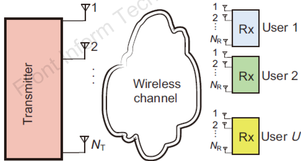
Fig. 5 Space–time wireless communication system
